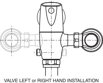
VALVE LEFT or RIGHT HAND INSTALLATION
